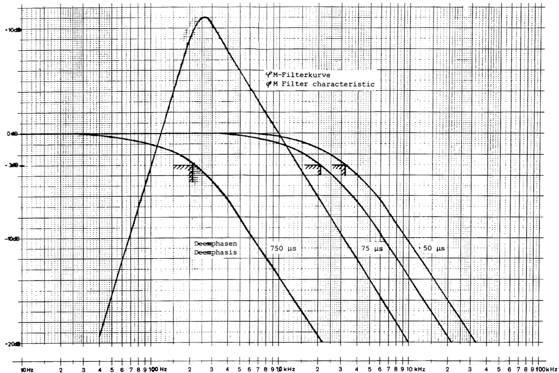
Bild 2-9 Deemphasen, \varphi M-Filterkurve Fig. 2-9 Deemphasis, \varphi M Filter characteristic
